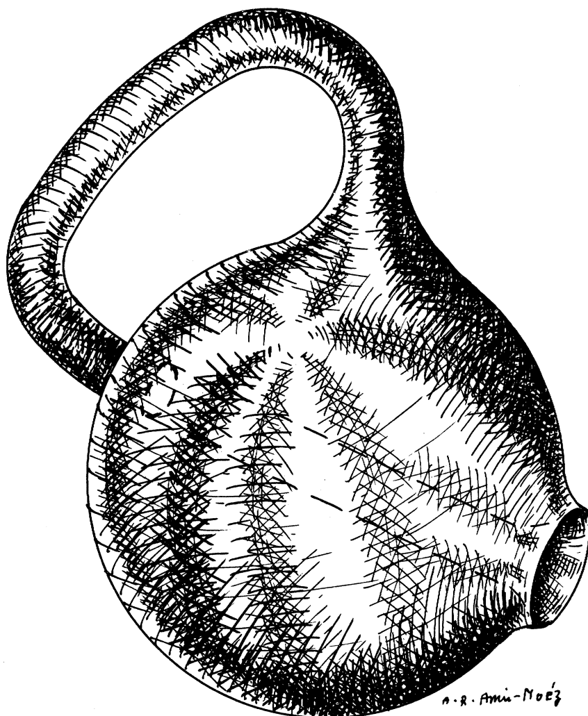
Klein bottle
